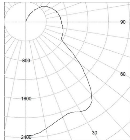
LDC: SL503C 200W
