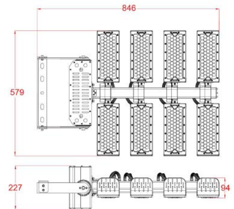
Dimension for SL-T500-960W
