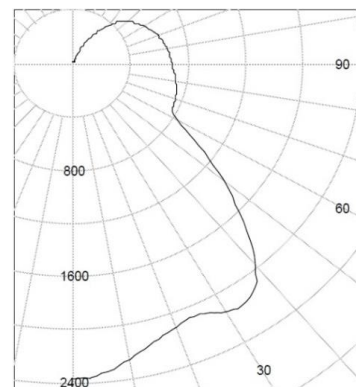
LDC: SL503/200C
